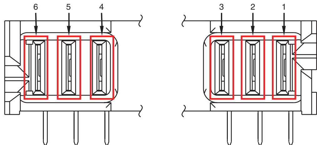
Figure 2-28: Z-DOK+ Utility Pins (ML410 Side)
